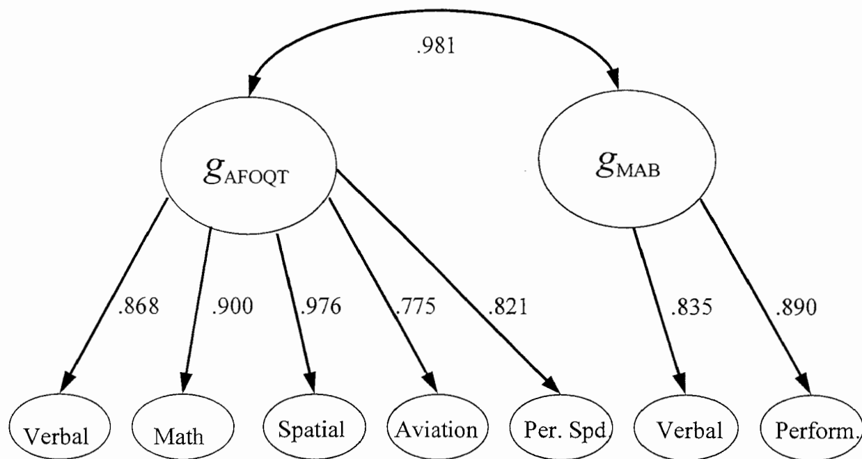
Figure 1. Hierarchical Model.
